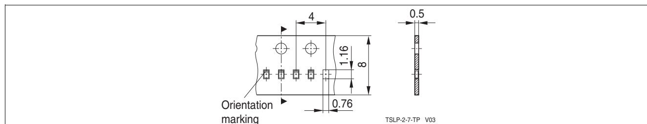
Figure 6-3 PG-TSLP-2-17: Packing
