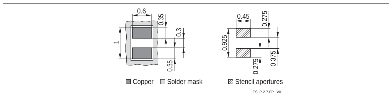
Figure 6-2 PG-TSLP-2-17: Footprint
