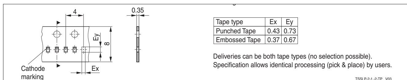
Figure 6-7 PG-TSSLP-2-1: Packing
