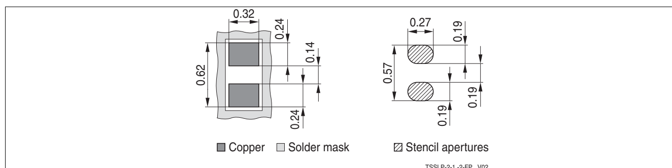
Figure 6-6 PG-TSSLP-2-1: Footprint
