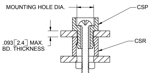
TYPICAL ASSEMBLY
