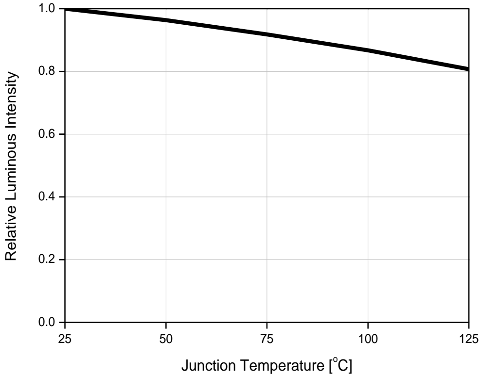
Fig 6. Junction Temperature vs. Relative Light Output, I_F=20mA
