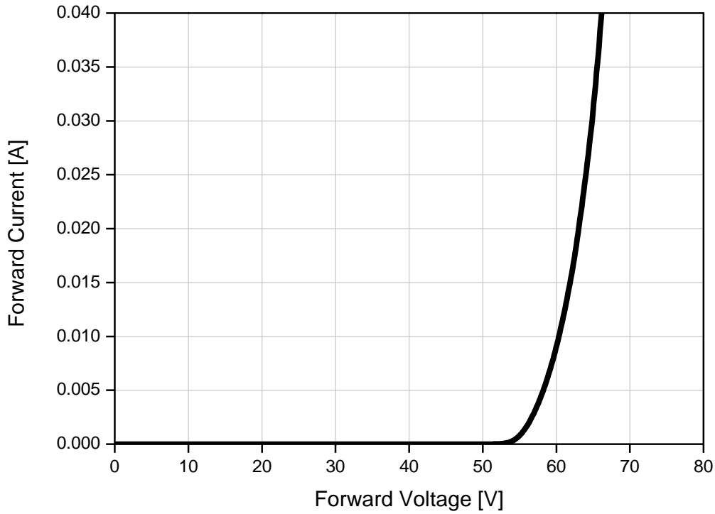
Fig 3. Forward Voltage vs. Forward Current, T_j = 25^\circ\text{C}
