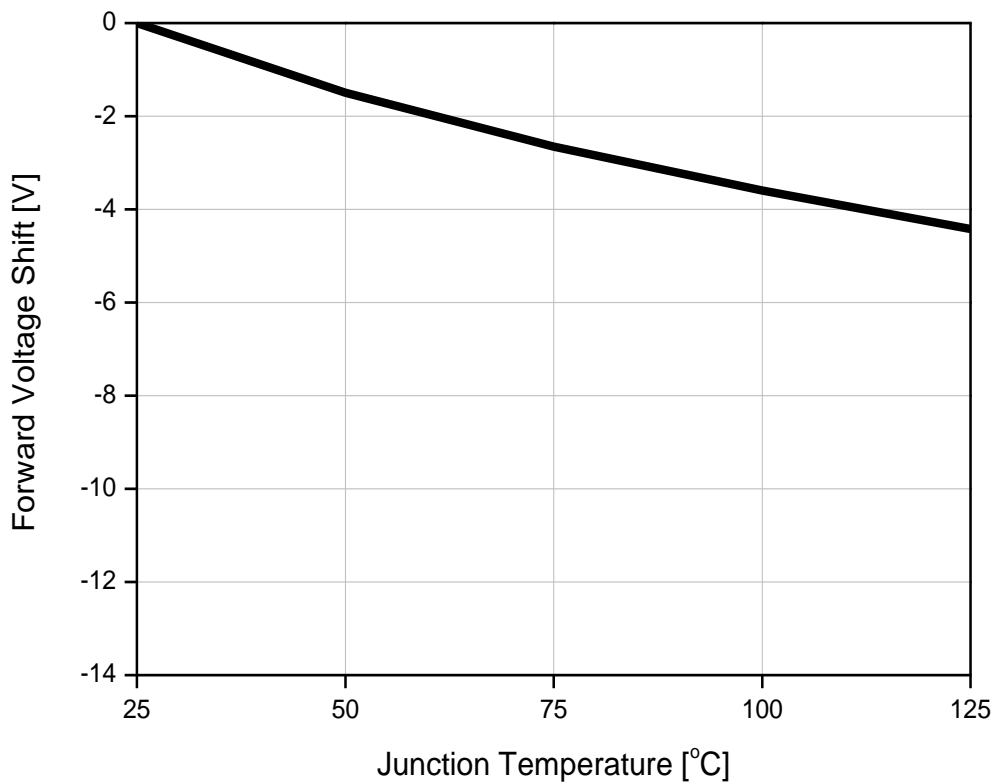
Fig 7. Junction Temperature vs. Relative Forward Voltage, I_F=20mA
