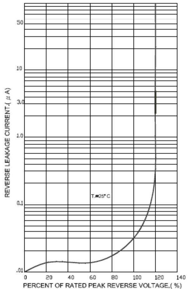
FIG.4-TYPICAL REVERSE CHARACTERISTICS
