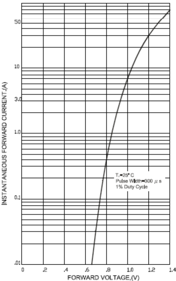
FIG.3-TYPICAL FORWARD CHARACTERISTICS
