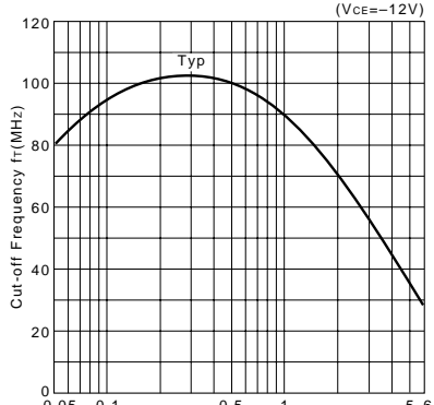
f T -I E Characteristics (Typical)
