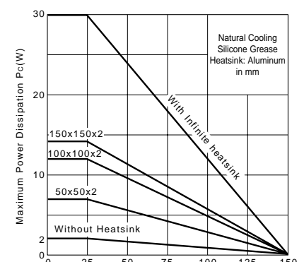
P C -T a Derating
