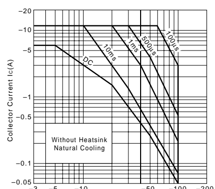
Safe Operating Area (Single Pulse)
