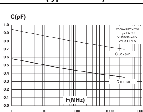
Figure 5. Line capacitance versus frequency (typical values)
