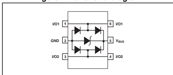
Figure 1. Functional diagram
