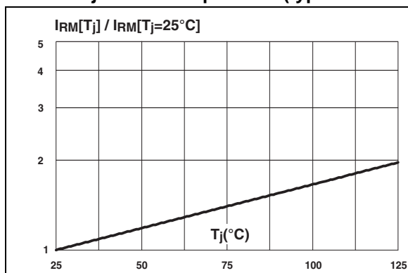
Figure 2. Relative variation of leakage current versus junction temperature (typical values)
