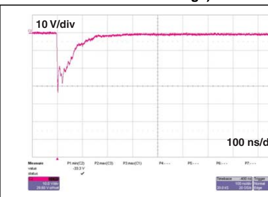
Figure 7. Remaining voltage on I/O2 after USBULC-2P6 during negative ESD surge (-15 kV air discharge)
