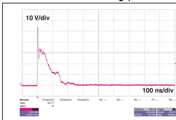
Figure 6. Remaining voltage on I/O1 after USBULC-2P6 during positive ESD surge (+15 kV air discharge)
