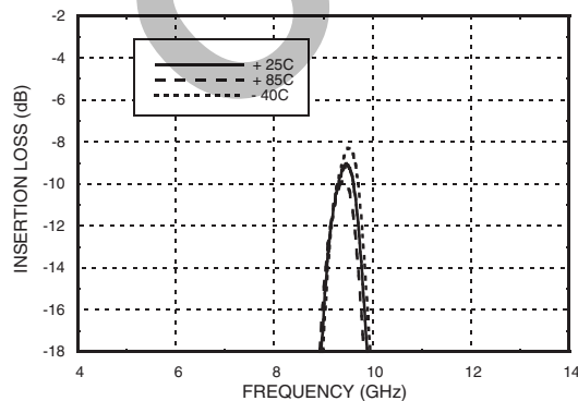
Insertion Loss vs. Temperature, V_{fctl} = V_{bwctl} = 7V
