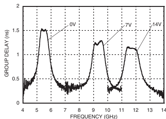
Group Delay, V_{ctl} = V_{bwctl}
