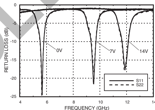
Return Loss vs. Control Voltages, V_{fctl} = V_{bwctl}
