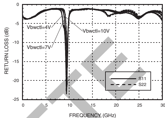
Broadband Return Loss vs. Vbwctl, Vfctl = 7V
