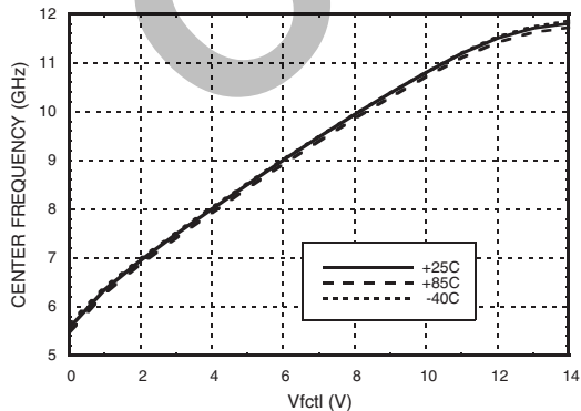
Center Frequency vs. Temperature, Vfctl = Vbwctl
