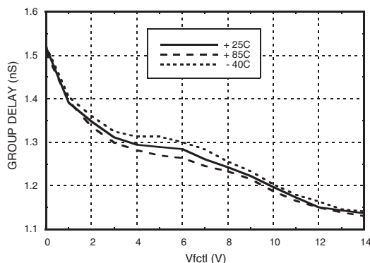
Group Delay vs. Fcenter vs. Temperature
