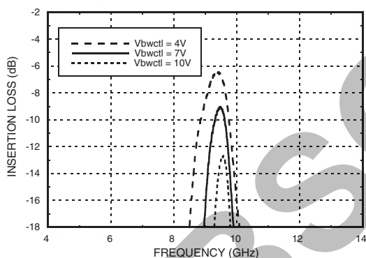
Insertion Loss vs. Vbwctl, Vfctl = 7V
