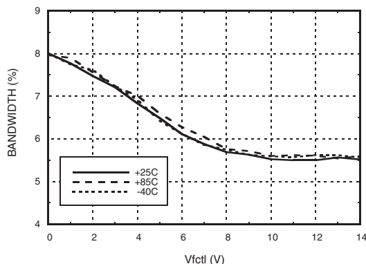
3 dB Bandwidth vs. Temperature, V_{fctl} = V_{bwctl}
