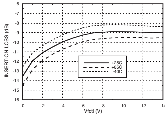
Insertion Loss vs. Temperature, Vfctl = Vbwctl
