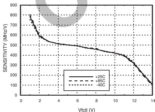
Tuning Sensitivity vs. Temperature, V_{fctl} = V_{bwctl}
