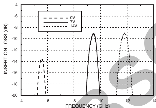
Insertion Loss vs. Control Voltages, V_{fctl} = V_{bwctl}
