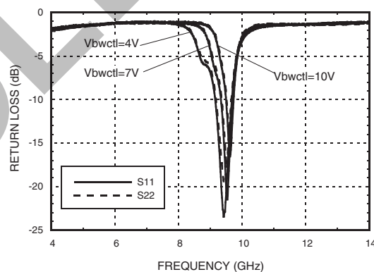
Return Loss vs. Vbwctl, Vfctl = 7V
