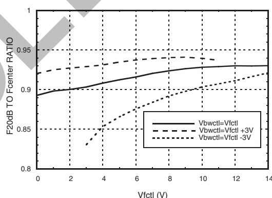
Low Side Rejection Ratio vs. Bandwidth Control [1]
