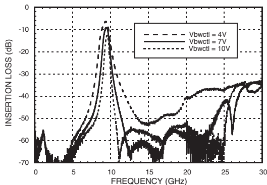
Broadband Insertion Loss vs. Vbwctl, Vfctl = 7V
