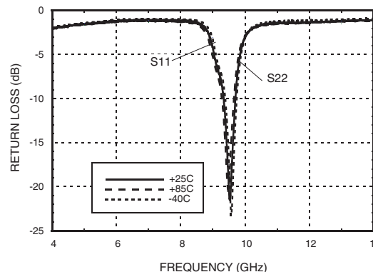
Return Loss vs. Temperature, V_{fctl} = V_{bwctl} = 7V
