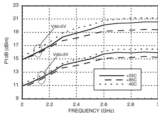
P1dB vs. Temperature [1] [2]
