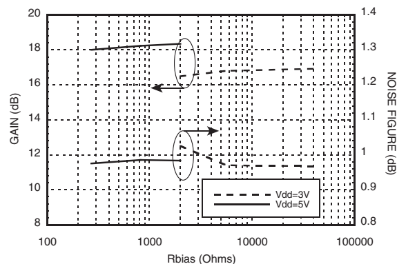
Gain, Noise Figure & Rbias @ 2700 MHz
