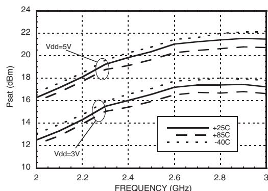
Psat vs. Temperature [1] [2]
