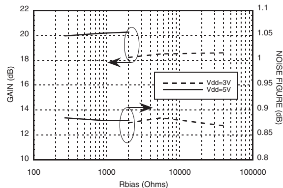
Gain, Noise Figure & Rbias @ 2300 MHz
