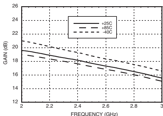
Gain vs. Temperature [2]
