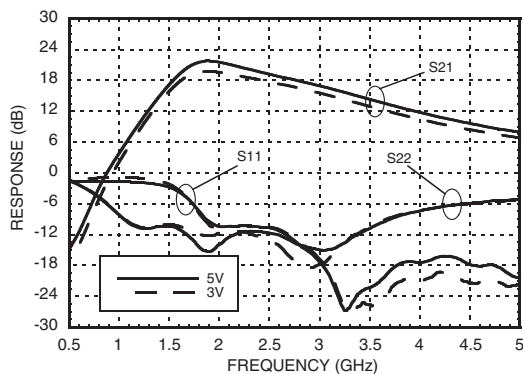
Broadband Gain & Return Loss [1] [2]
