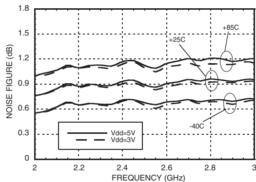
Noise Figure vs. Temperature [1] [2] [4]
