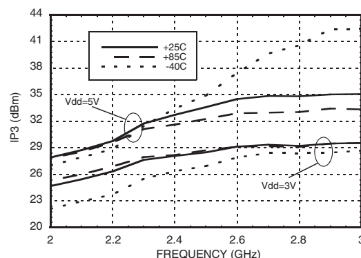
Output IP3 vs. Temperature [1] [2]
