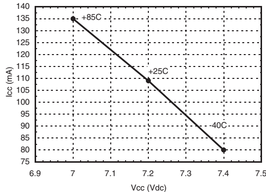
Vcc vs. Icc Over Temperature for Fixed Vs= 8V, RBIAS= 9.1 Ohms
