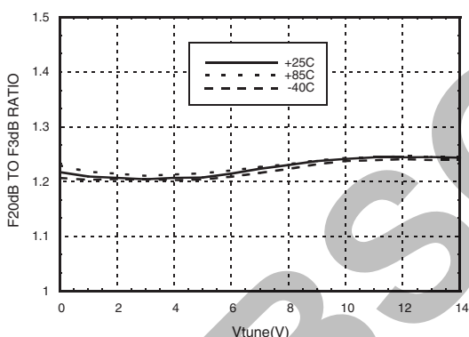
Rejection Ratio vs. Temperature [1]
