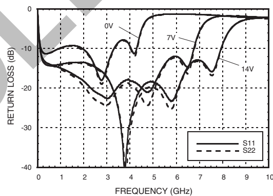
Return Loss vs. Control Voltage [1]
