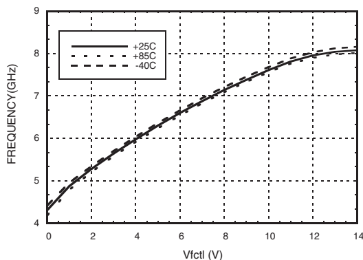
Cutoff Frequency vs. Temperature
