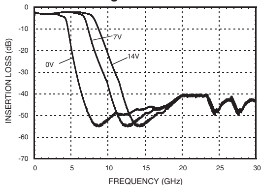
Broadband Insertion Loss vs. Control Voltage
