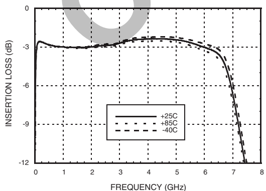
Insertion Loss vs. Temperature, Vfctl @ 7V [1]
