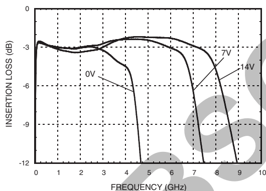
Insertion Loss vs. Control Voltage [1]
