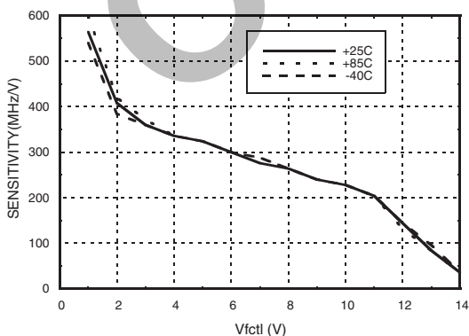
Tuning Sensitivity vs. Temperature
