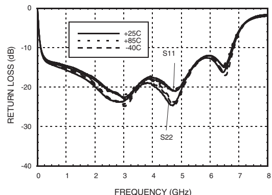
Return Loss vs. Temperature, Vfctl @ 7V [1]
