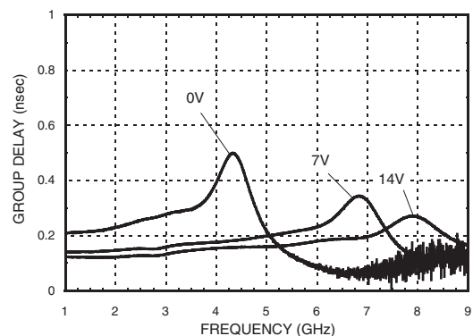
Group Delay
