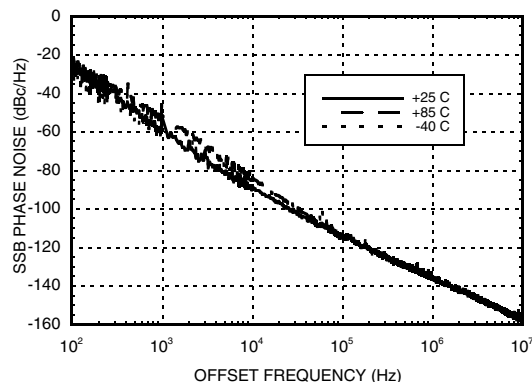
SSB Phase Noise @ V_{tune} = +5\text{V}
