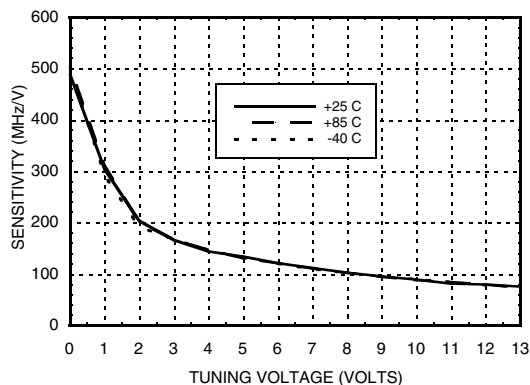
Sensitivity vs. Tuning Voltage, V_{cc} = +5\text{V}
