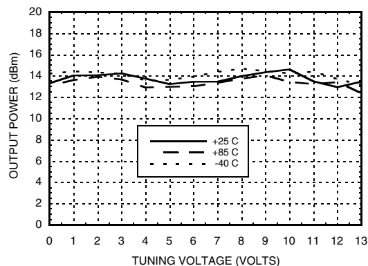
Output Power vs. Tuning Voltage, V_{cc} = +5\text{V}
