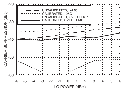
Carrier Suppression* vs. LO Power@ 2100 MHz
