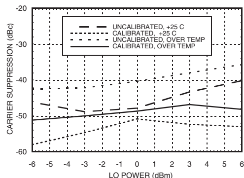
Carrier Suppression* vs. LO Power@ 1900 MHz
