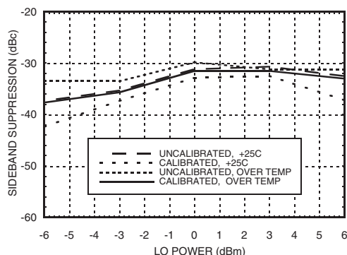
Sideband Suppression* vs. LO Power@ 2100 MHz
