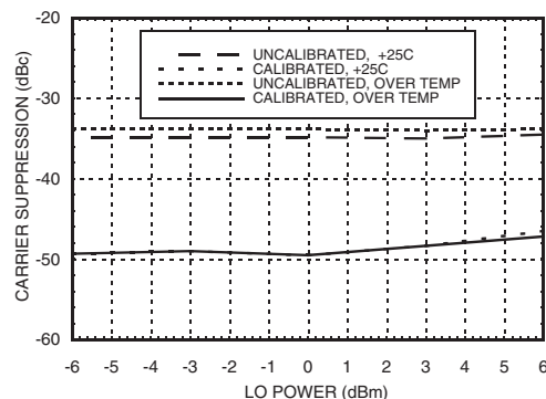
Carrier Suppression* vs. LO Power@ 830 MHz
