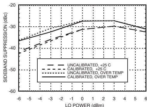
Sideband Suppression* vs. LO Power@ 1900 MHz
