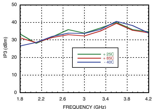
Input IP3 vs. Temperature @ LO = 4 dBm
