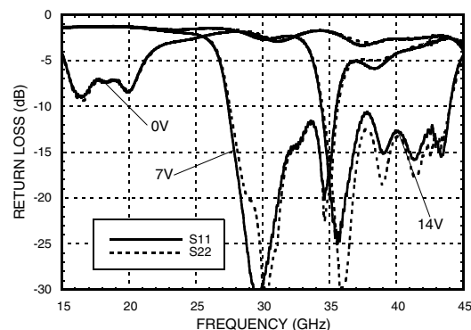
Return Loss vs. Vfctl
