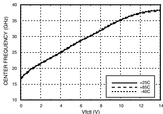
Center Frequency vs. Temperature
