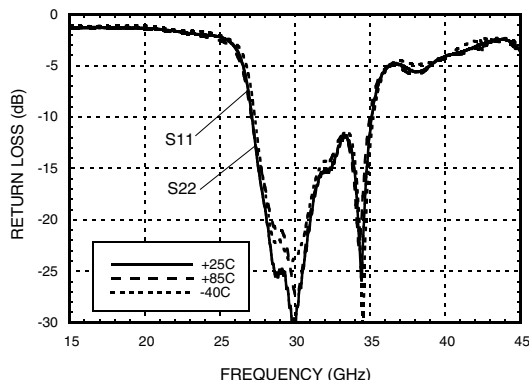
Return Loss vs. Temperature, Vfctl = 7V
