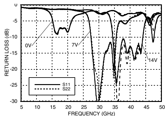
Broadband Return Loss vs. Vfctl
