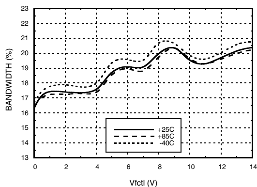
3 dB Bandwidth vs. Temperature
