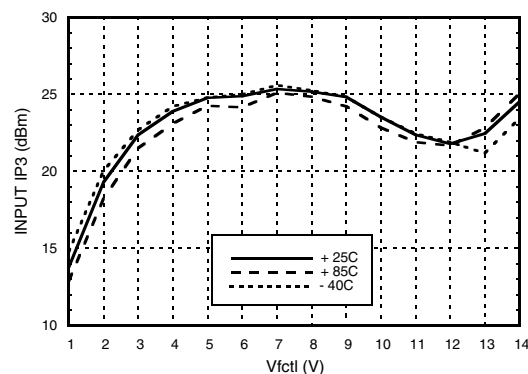
Input IP3 vs. Temperature
