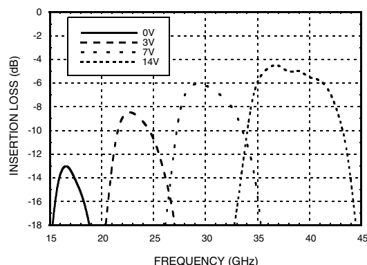
Insertion Loss vs. Vfctl
