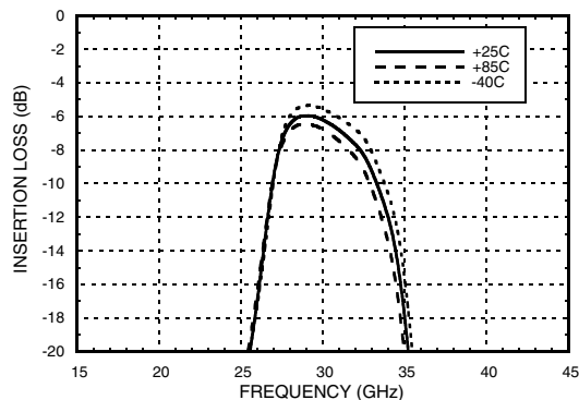
Insertion Loss vs. Temperature, Vfctl = 7V
