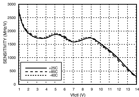
Tuning Sensitivity vs. Temperature
