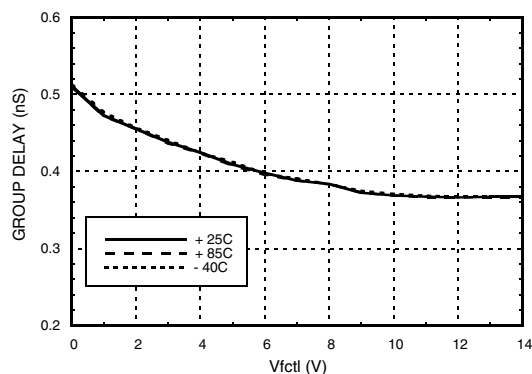
Group Delay vs. Fcenter vs. Temperature
