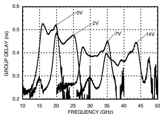
Group Delay
