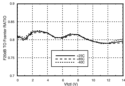
Low Side Rejection Ratio vs. Temperature [1]
