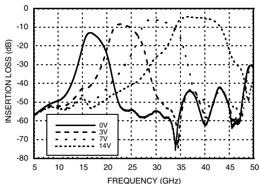
Broadband Insertion Loss vs. Vfctl
