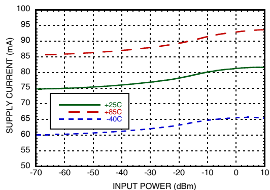
Typical Supply Current vs. Pin, Vcc = 5V
