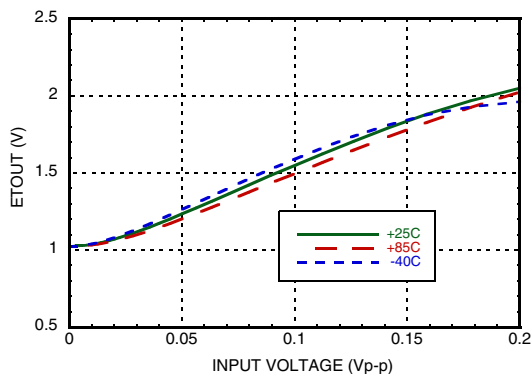
ETOUT vs. Pin with CW @ 3500 MHz
