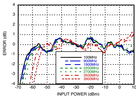
RMSOUT Error vs. Pin with CW @ +25 °C [1]
