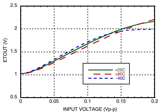
ETOUT vs. Pin with CW @ 1900 MHz
