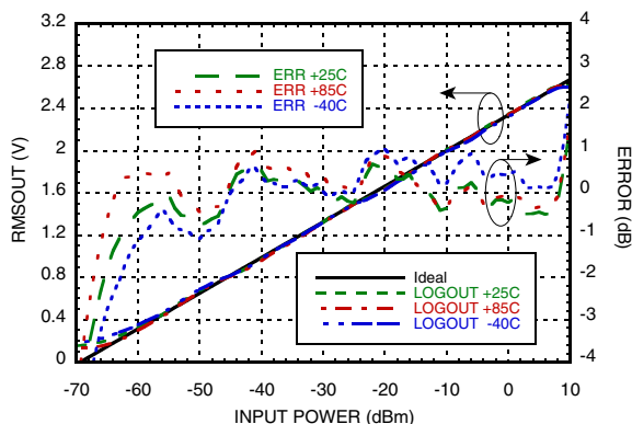
RMSOUT & Error vs. Pin @ 100 MHz [1][2]
