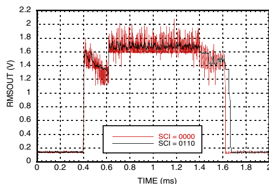
Residual Ripple for 900 MHz LTE Downlink @ SCI=0110
