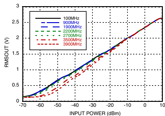
RMSOUT vs. Pin with WCDMA 4 Carrier @ +25 °C [1]
