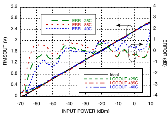
RMSOUT & Error vs. Pin @ 1900 MHz [1][2]
