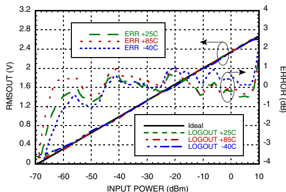
RMSOUT & Error vs. Pin @ 900 MHz [1][2]
