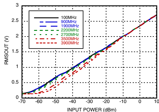
RMSOUT vs. Pin with CW @ +25 °C [1]
