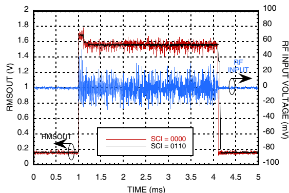
Residual Ripple for 900 MHz WiBro @ SCI=0110
