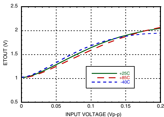
ETOUT vs. Pin with CW @ 900 MHz
