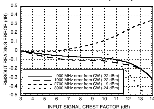
RMSOUT Error vs. Crest Factor over Frequency
