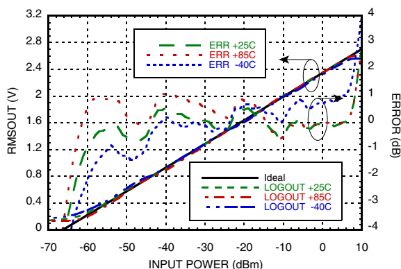
RMSOUT & Error vs. Pin @ 2700 MHz [1][2]
