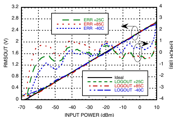
RMSOUT & Error vs. Pin @ 2200 MHz [1][2]
