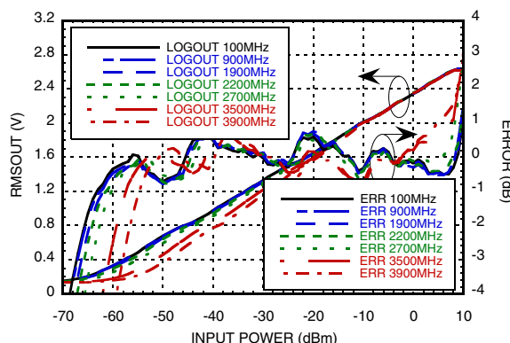
RMSOUT & Error vs. Pin
