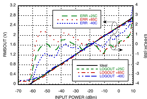
RMSOUT & Error vs. Pin @ 3500 MHz [1][2]
