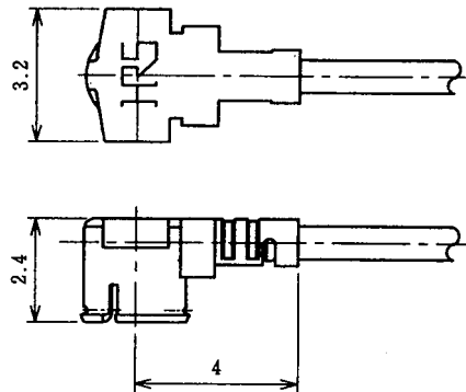
Diagram of the Condition Following Cable Wiring
