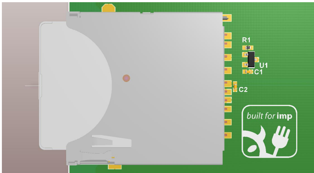
3: imp001 recommended layout in 3D, board top
