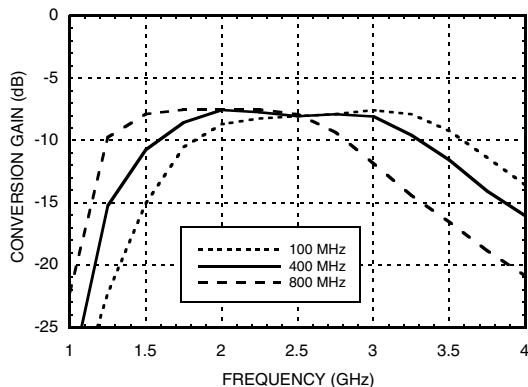
Conversion Gain vs. IF Frequency
