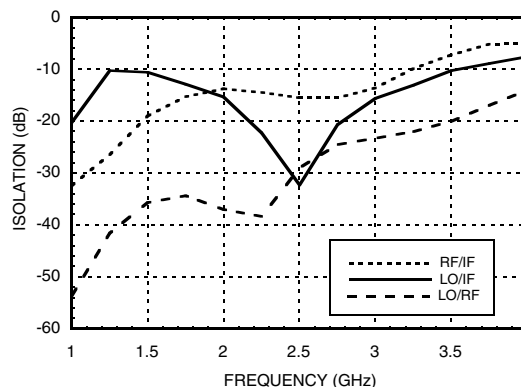
Isolation @ LO = +10 dBm
