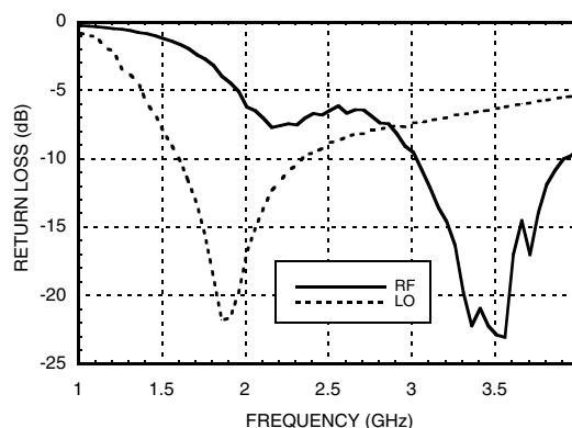
Return Loss @ LO = +10 dBm
