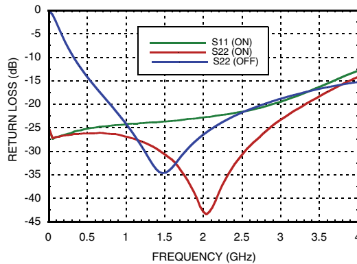
Return Loss
