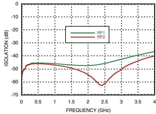
Isolation
