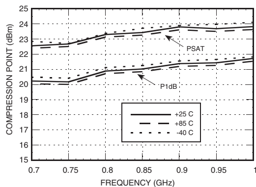
P1dB & Psat vs. Temperature
