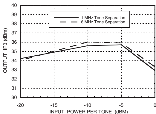
Output IP3 vs. Input Power @ 950 MHz
