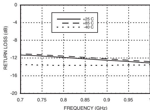
LNA Output Return Loss vs. Temperature
