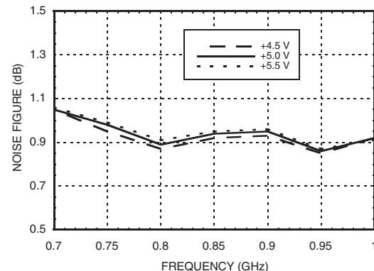
LNA Noise Figure vs. Vdd
