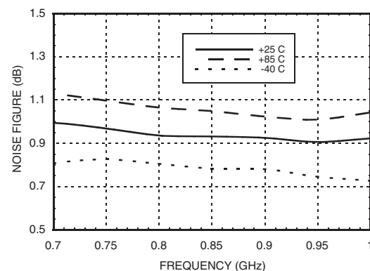
LNA Noise Figure vs. Temperature
