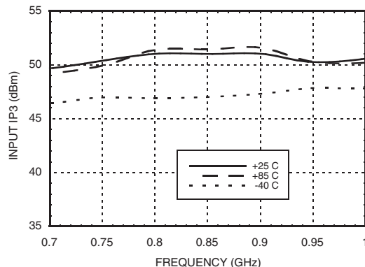
Bypass Mode Input IP3 vs. Temperature
