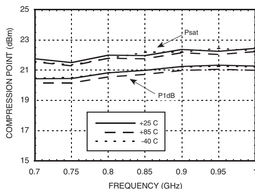
LNA P1dB & Psat vs. Temperature
