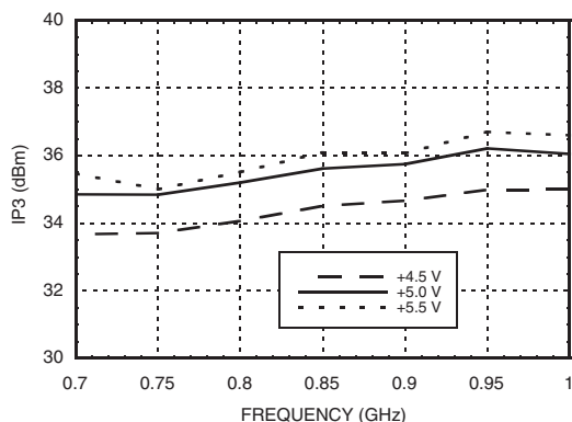
LNA Output IP3 vs. Vdd
