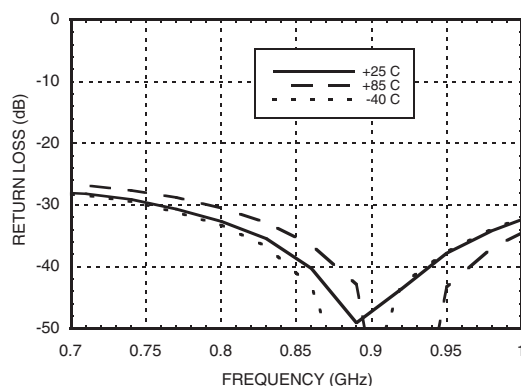
Bypass Mode Input Return Loss vs. Temperature
