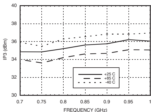
LNA Output IP3 vs. Temperature
