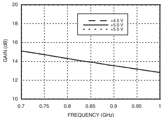
LNA Gain vs. Vdd
