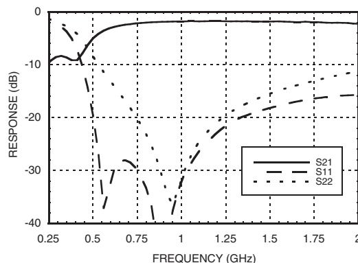
Bypass Mode Broadband Insertion Loss & Return Loss
