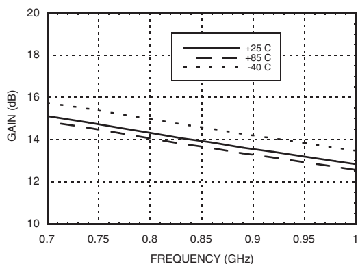
LNA Gain vs. Temperature
