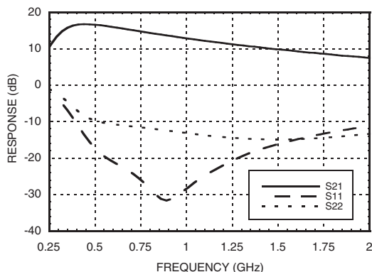
LNA Broadband Gain & Return Loss
