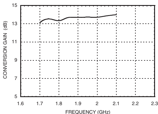
Conversion Gain with IF Tuned for 70 MHz
