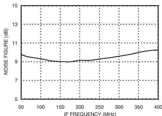
Noise Figure Swept IF, Fixed LO = 1.7 GHz
