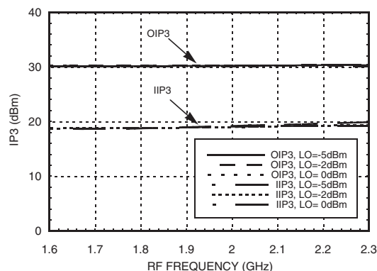
Input and Output IP3 vs LO Drive
