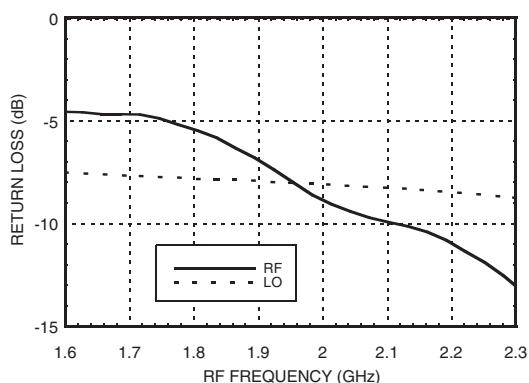
Return Loss
