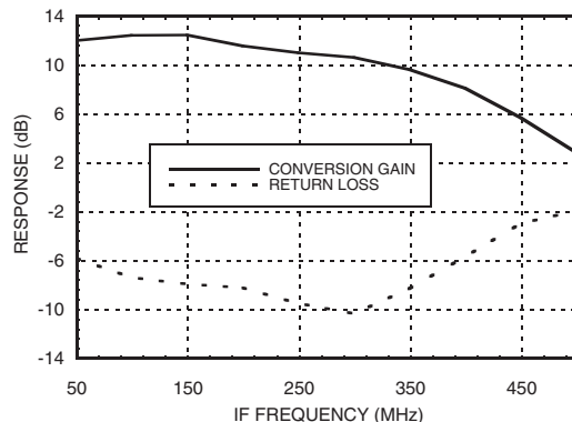
IF Bandwidth
