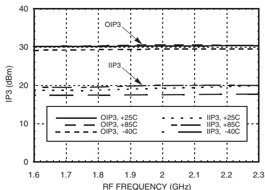
Input and Output IP3 vs. Temperature
