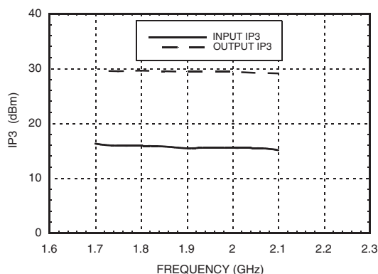
IP3 with IF Tuned for 70 MHz
