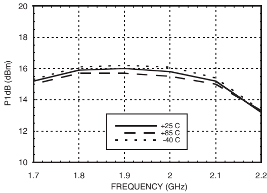
P1dB vs. Temperature @ Idd = 67 mA
