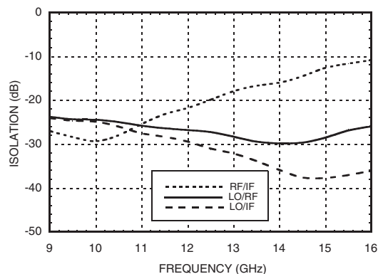
Isolation @ LO = +13 dBm
