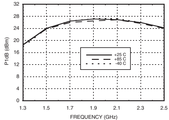
P1dB vs. Temperature, Vs= 5V
