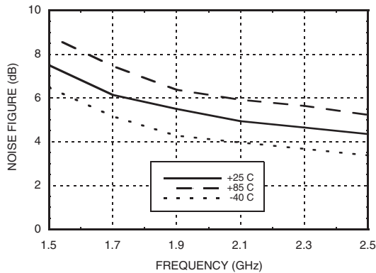
Noise Figure vs. Temperature, V_s = 3.6V
