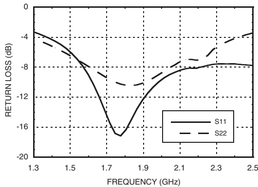
Return Loss, Vs= 3.6V
