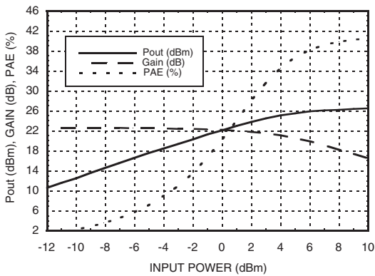
Power Compression@ 1.9 GHz, Vs= 3.6V
