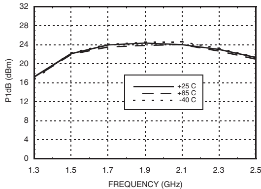
P1dB vs. Temperature, Vs= 3.6V
