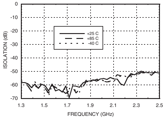
Reverse Isolation vs. Temperature, V_s = 3.6V
