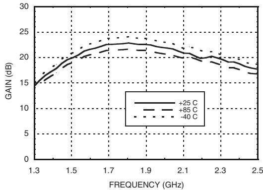
Gain vs. Temperature, Vs= 3.6V
