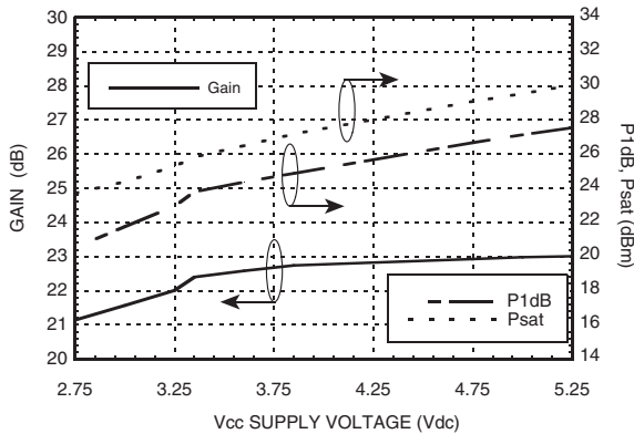
Gain & Power vs. Supply Voltage @ 1.9 GHz
