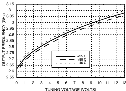
Divide-by-4 Frequency vs. Tuning Voltage, Vcc= +3V
