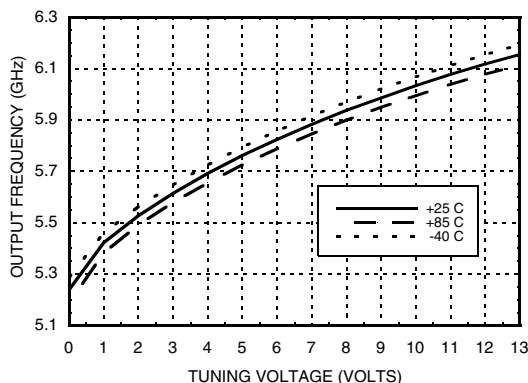
RFOUT/2 Frequency vs. Tuning Voltage, Vcc= +3V
