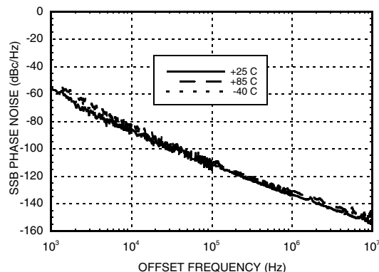
SSB Phase Noise @ V_{\text{tune}} = +5\text{V}
