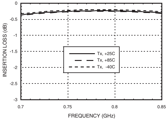
Insertion Loss vs. Temperature, Tx with 785 MHz Tuning
