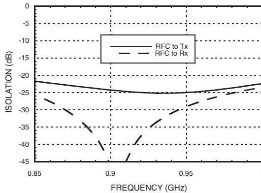
Isolation with 915 MHz Tuning
