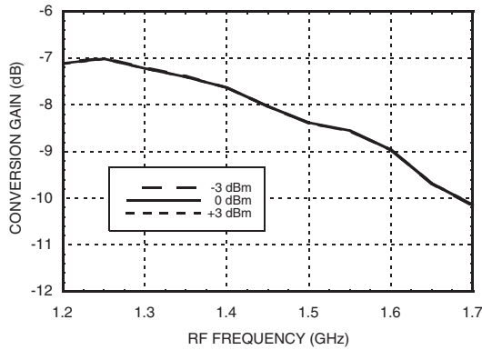
Upconverter Performance Conversion Gain vs. LO Drive [2]
