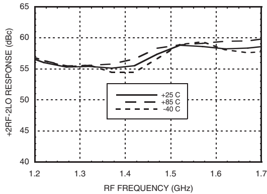
+2RF -2LO Response vs. Temperature [2] [4]
