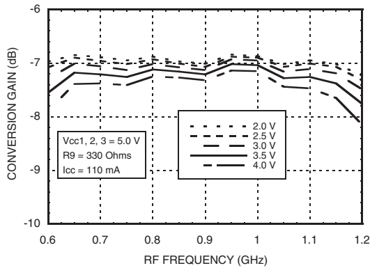
Conversion Gain vs. G_Bias Voltage
