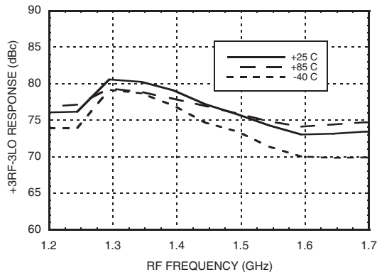
+3RF -3LO Response vs. Temperature [2] [4]
