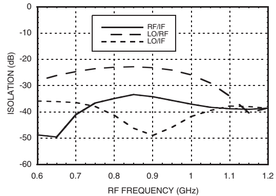
Isolation
