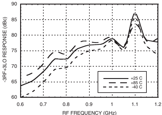
-3RF +3LO Response vs. Temperature [2]
