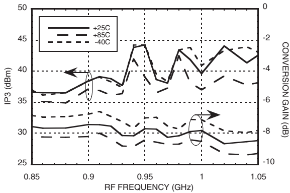
Conversion Gain and IP3, G_BIAS = 1.5 [2][3]
