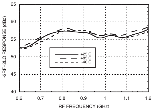
-2RF +2LO Response vs. Temperature [2]
