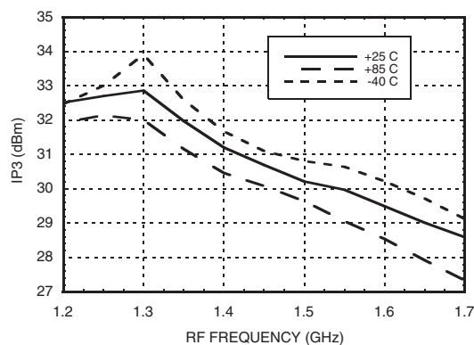
Upconverter Performance Input IP3 vs. Temperature [2] [3]
