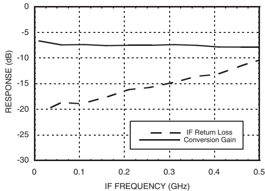
IF Bandwidth (LO = 1.1 GHz)
