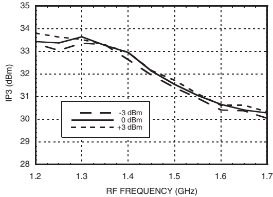
Input IP3 vs. LO Drive [2] [3]
