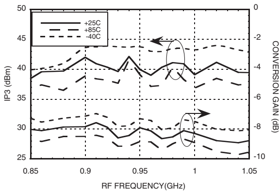
Conversion Gain and IP3, G_BIAS = 3.5 [2][3]
