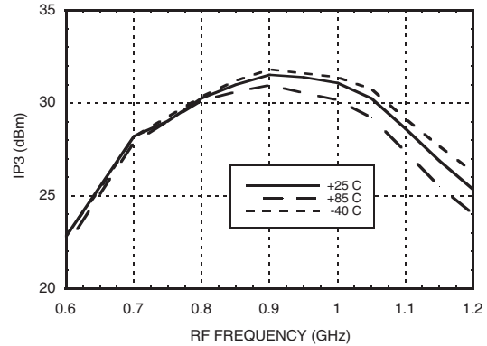
Input IP3 vs. Temperature, I_{cc} = 60\text{ mA} [1]
