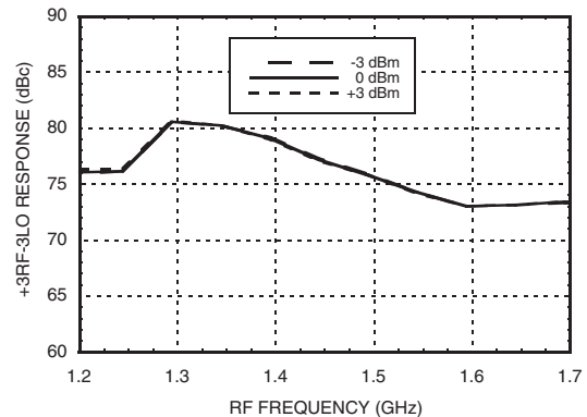
+3RF -3LO Response vs. LO Drive [2] [4]
