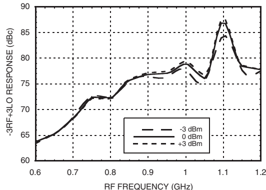
-3RF +3LO Response vs. LO Drive [2]
