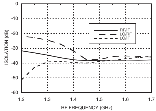
Isolation [2]
