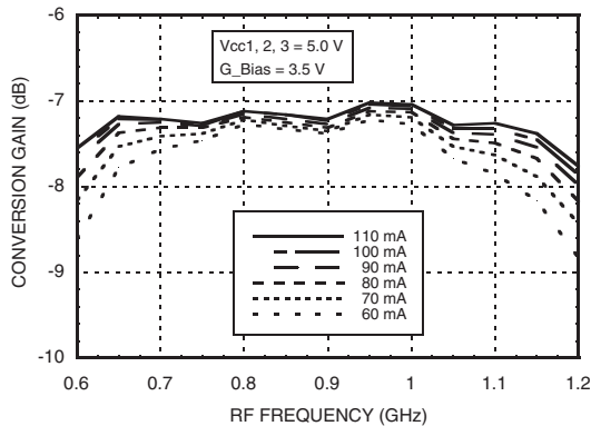
Conversion Gain vs. Icc
