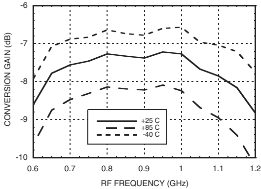
Conversion Gain vs. Temperature, I_{cc} = 60\text{ mA}
