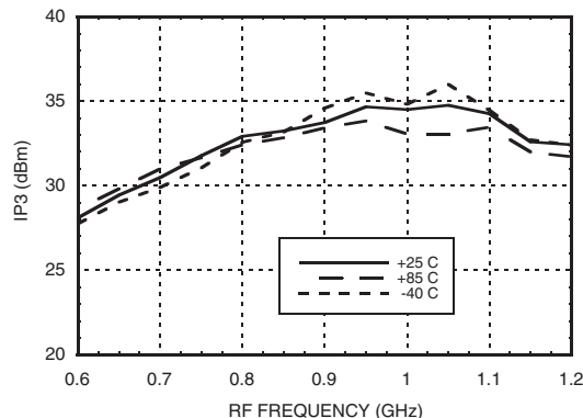
Input IP3 vs. Temperature [1]
