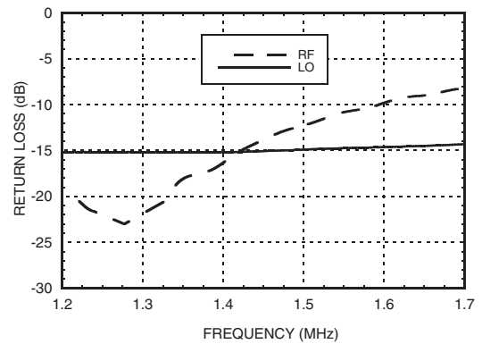
Return Loss
