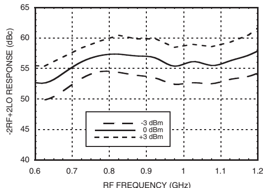
-2RF +2LO Response vs. LO Drive [2]
