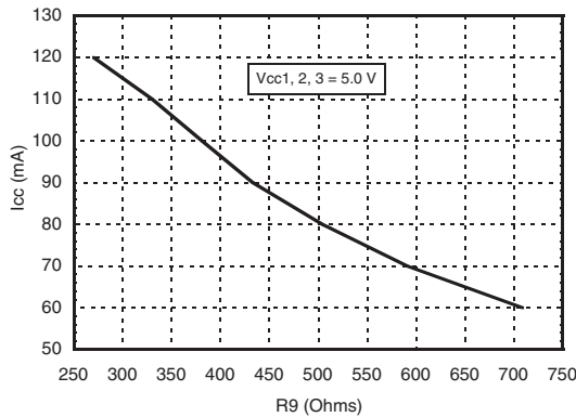
I_{cc} vs. R9
