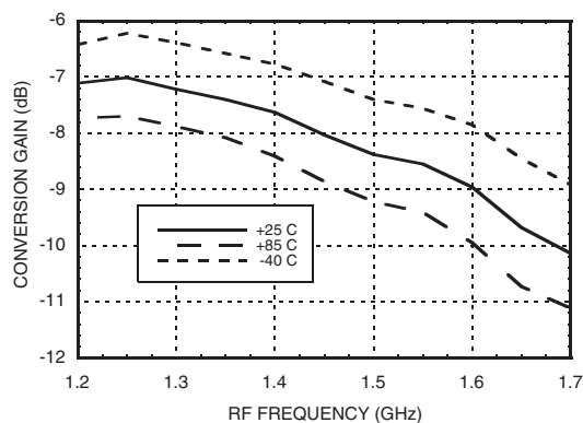
Upconverter Performance Conversion Gain vs. Temperature [3]
