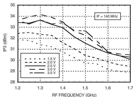
Input IP3 vs. G_Bias Voltage [2]
