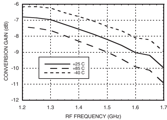
Conversion Gain vs. Temperature [2]
