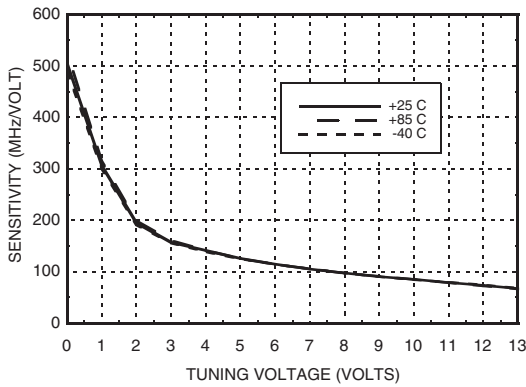
Sensitivity vs. Tuning Voltage, Vcc = +4.2V
