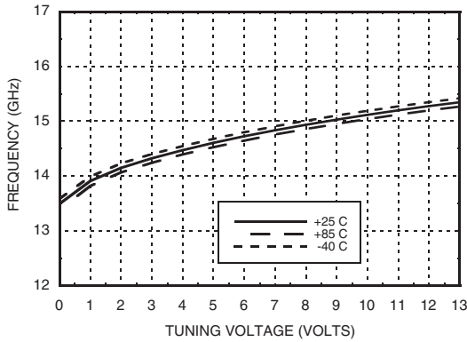
Frequency vs. Tuning Voltage, Vcc = +4.2V
