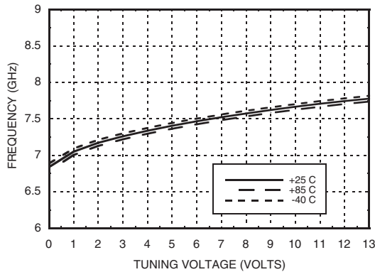
RFOUT/2 Frequency vs. Tuning Voltage, Vcc = +4.2V
