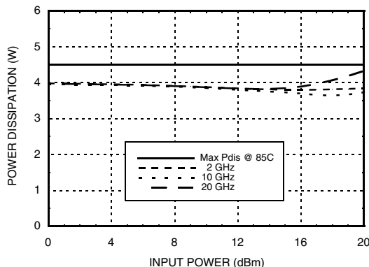
Power Dissipation
