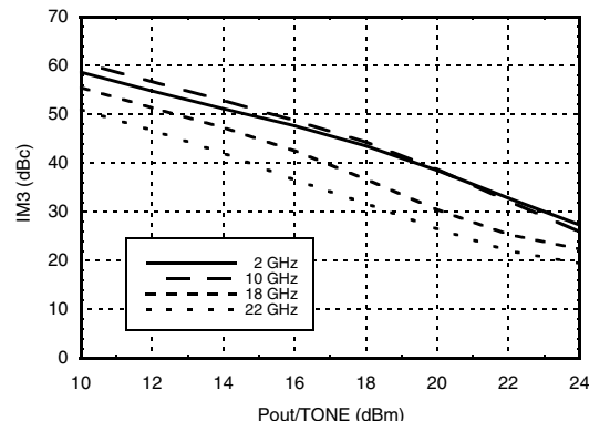
Output IM3 @ Vdd = +11V
