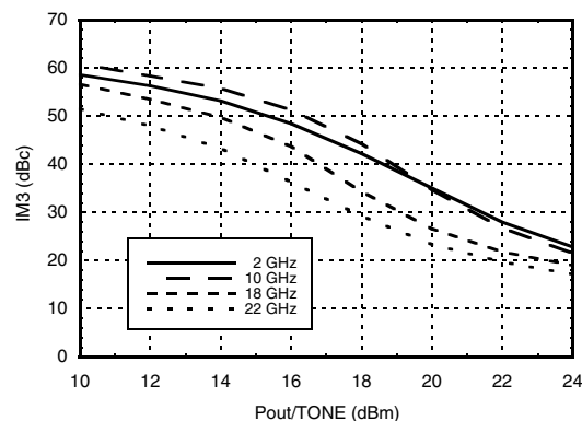
Output IM3 @ Vdd = +8V
