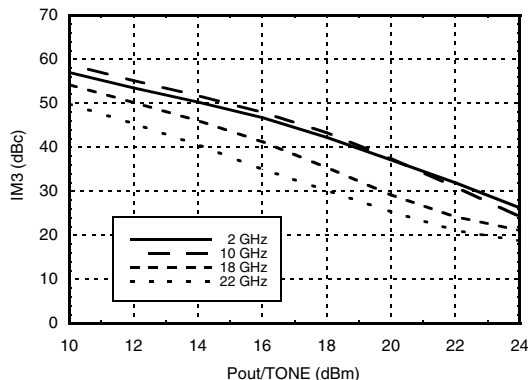
Output IM3 @ Vdd = +10V
