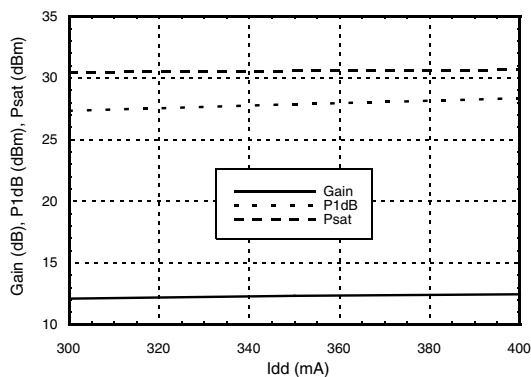
Gain & Power vs. Supply Current @ 10 GHz
