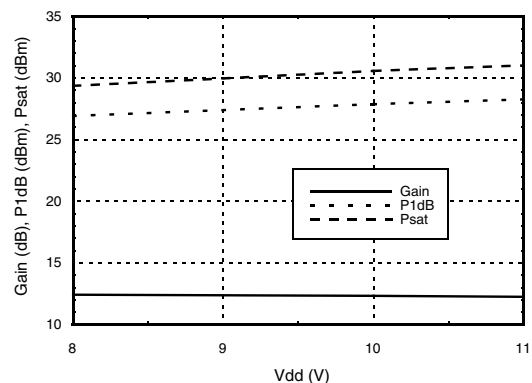
Gain & Power vs. Supply Voltage @ 10 GHz
