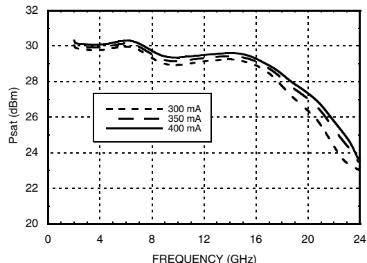
Psat vs. Supply Current
