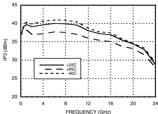
Output IP3 vs. Temperature @ Pout = 18 dBm / Tone
