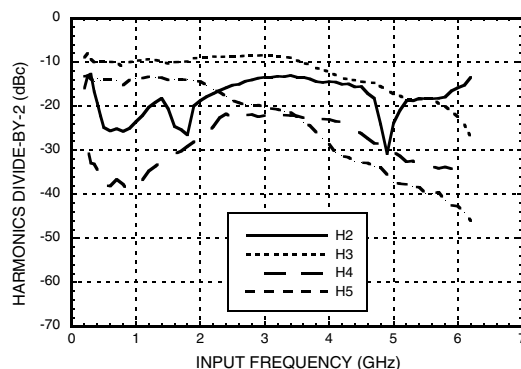
H2, H3, H4, H5 Harmonics, Divide-by-2 [1]
