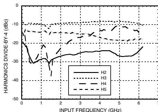
H2, H3, H4, H5 Harmonics, Divide-by-4 [1]
