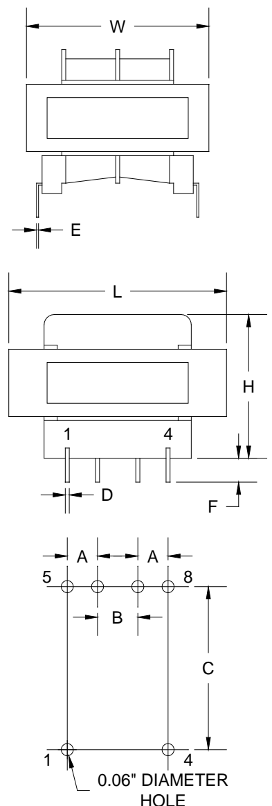
Board Layout
