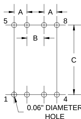
Board Layout
