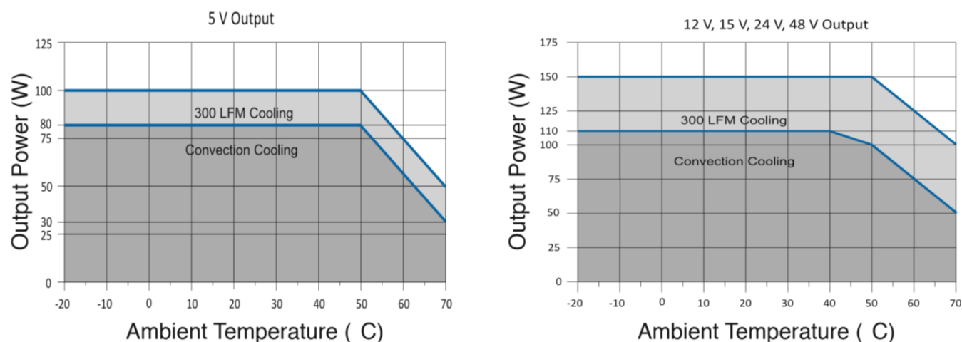
Figure 1 - Output Power Vs. Temperature
