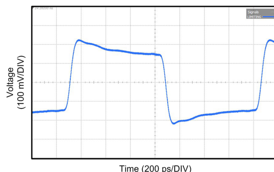
Figure 10. Example of TX De-emphasis for a DS125RT410 Operating at 10.3125 Gbps
