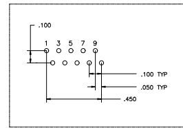
PIN DESIGNATIONS
