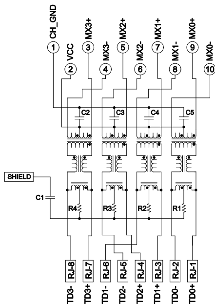
7G05 GIGABIT SCHEMATIC
