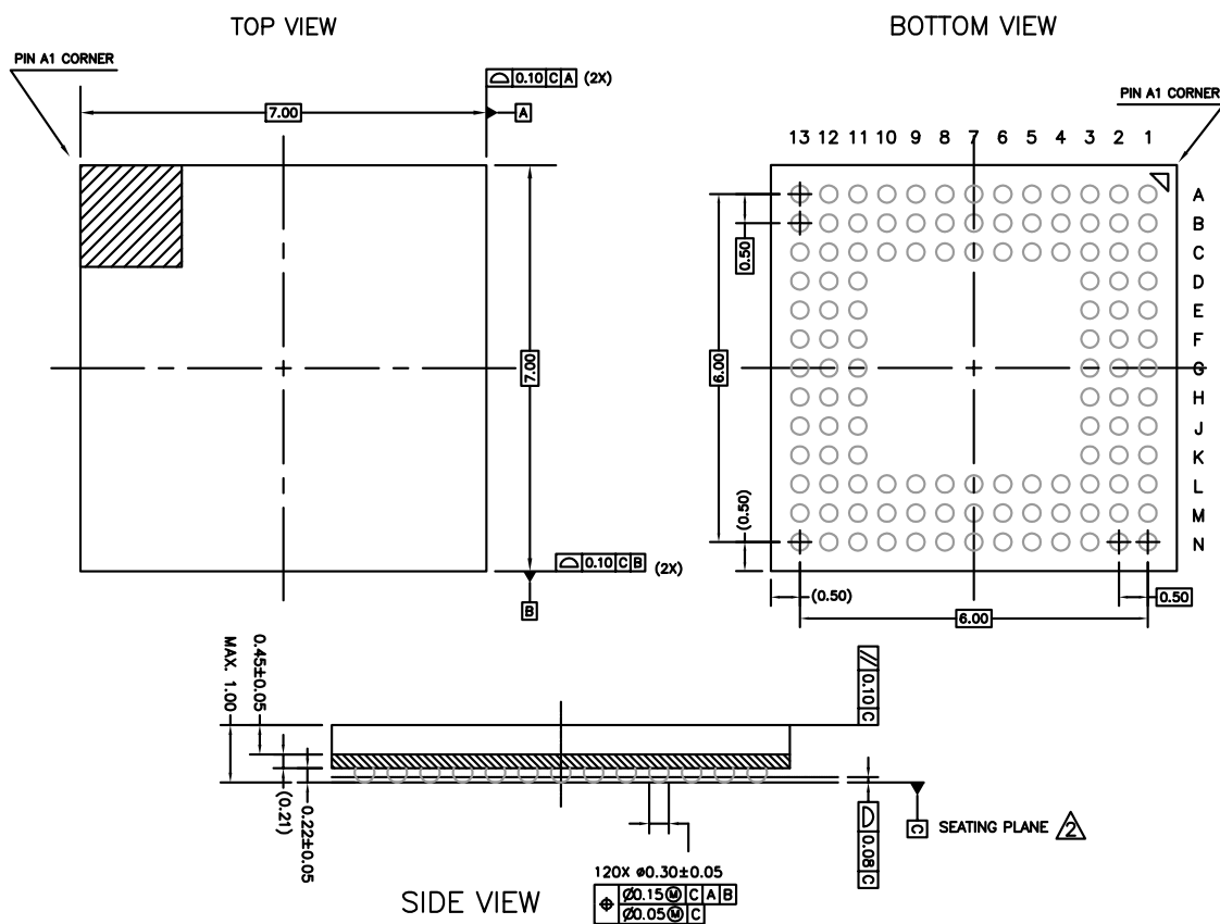
Figure 4.3. BGA120
