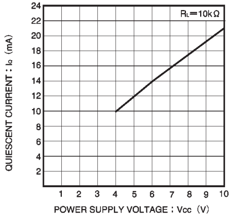
Fig. 3 Quiescent curve vs. power supply voltage
