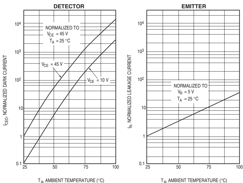
Figure 4. Leakage Current vs. Temperature
