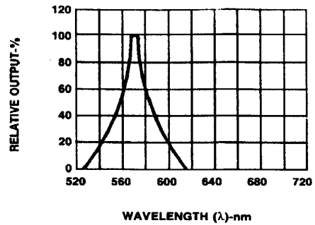
Fig.2 SPECTRAL RESPONSE
