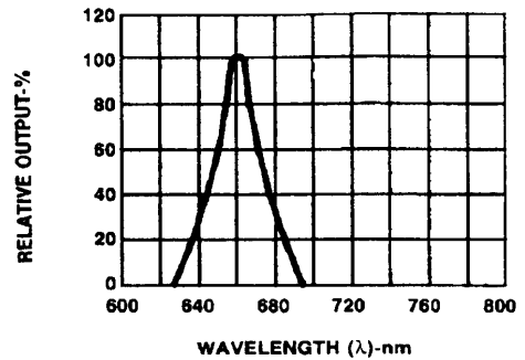
Fig.2 SPECTRAL RESPONSE
