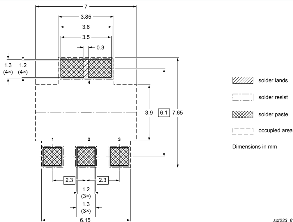
Fig. 19. Reflow soldering footprint for SC-73 (SOT223)
