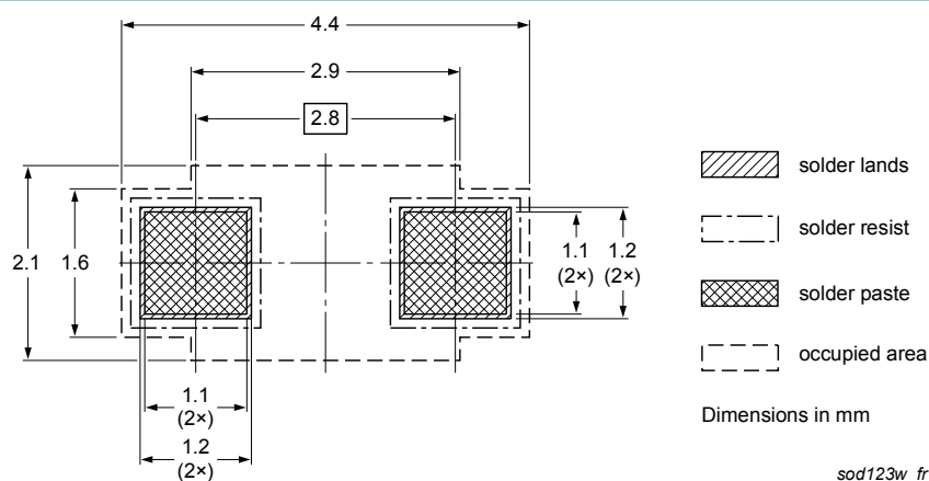
Fig. 19. Reflow soldering footprint for SOD123W
