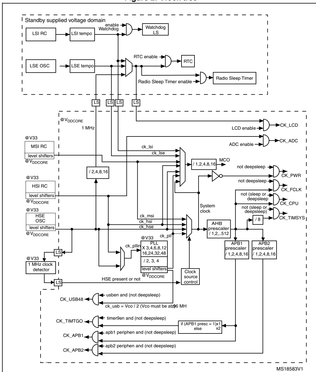
Figure 2. Clock tree
