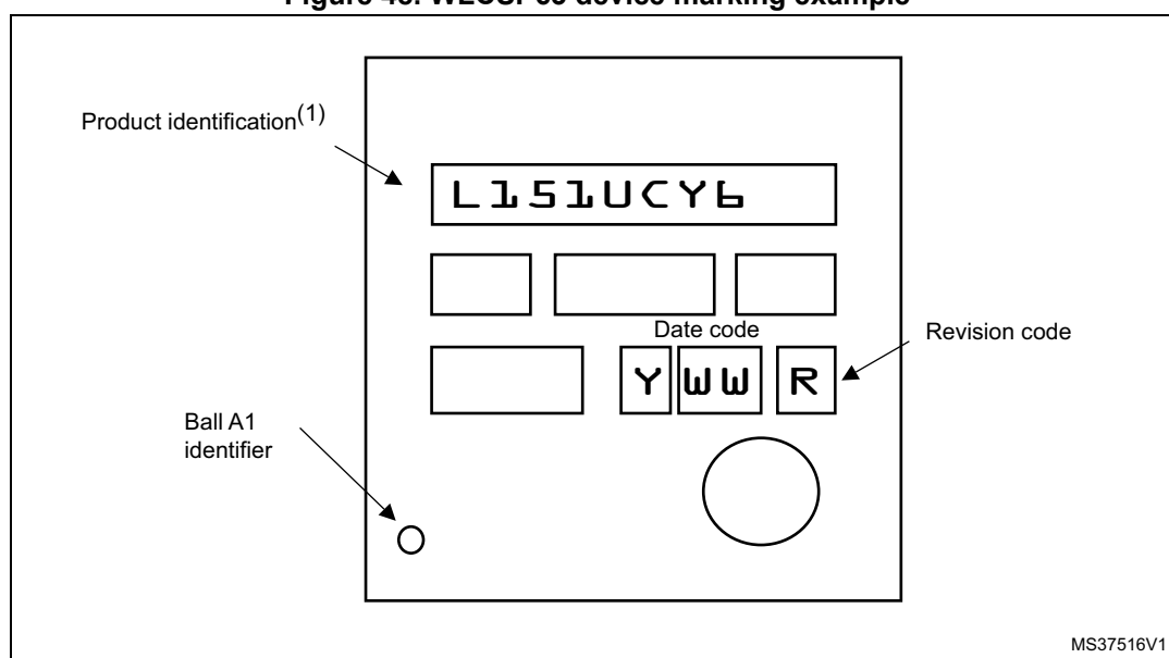
Figure 48. WLCSP63 device marking example
