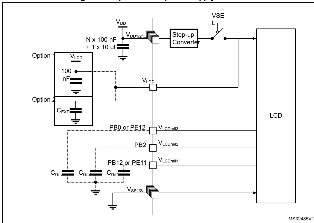
Figure 13. Optional LCD power supply scheme
