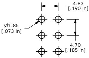
▲ PC MOUNTING
