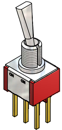
ISOMETRIC
