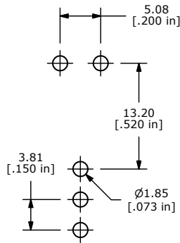
PCB MOUNTING LAYOUT
