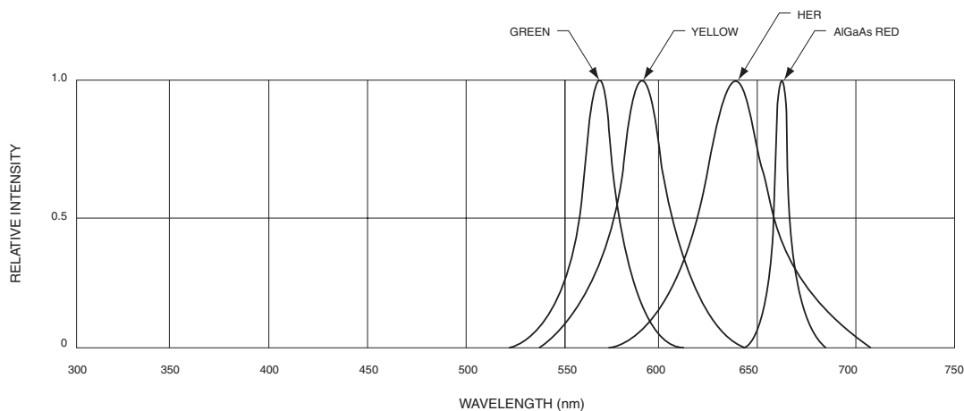
Fig.4 Radiation Diagram
