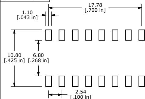
P.C.B. MOUNTING
