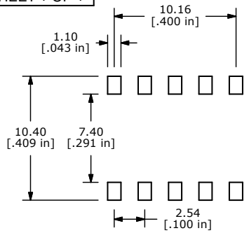
P.C.B. MOUNTING
