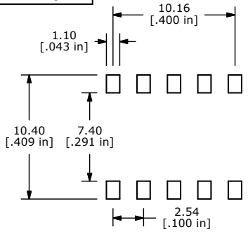
P.C.B. MOUNTING
