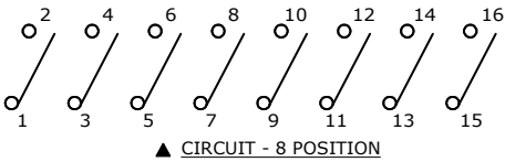
▲ CIRCUIT - 8 POSITION
